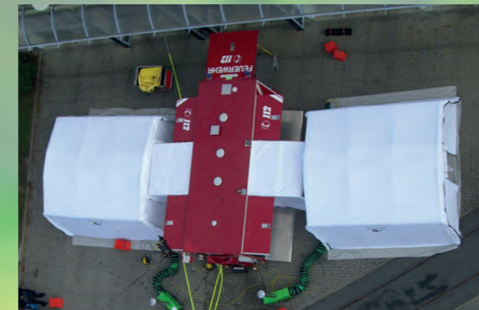
Ro/Ro container decontamination with dress and undress tent
